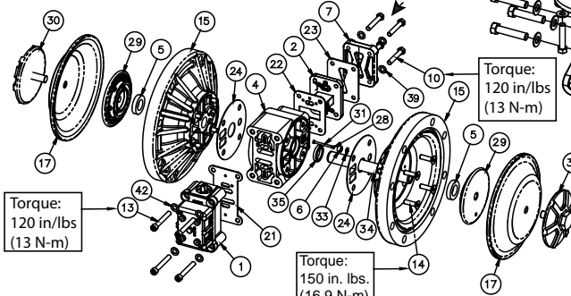
Air End Section Assembly
